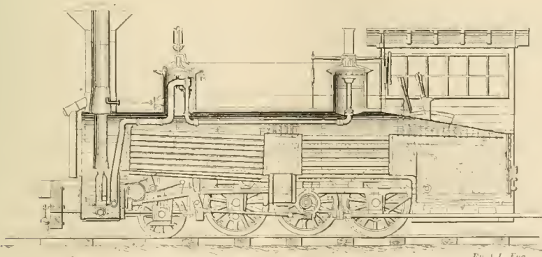
MILLHOLLAND'S 6 WHEEL CONNECTED ENGINE WITH HIS PATENTED BOILER. FIG. 77.
